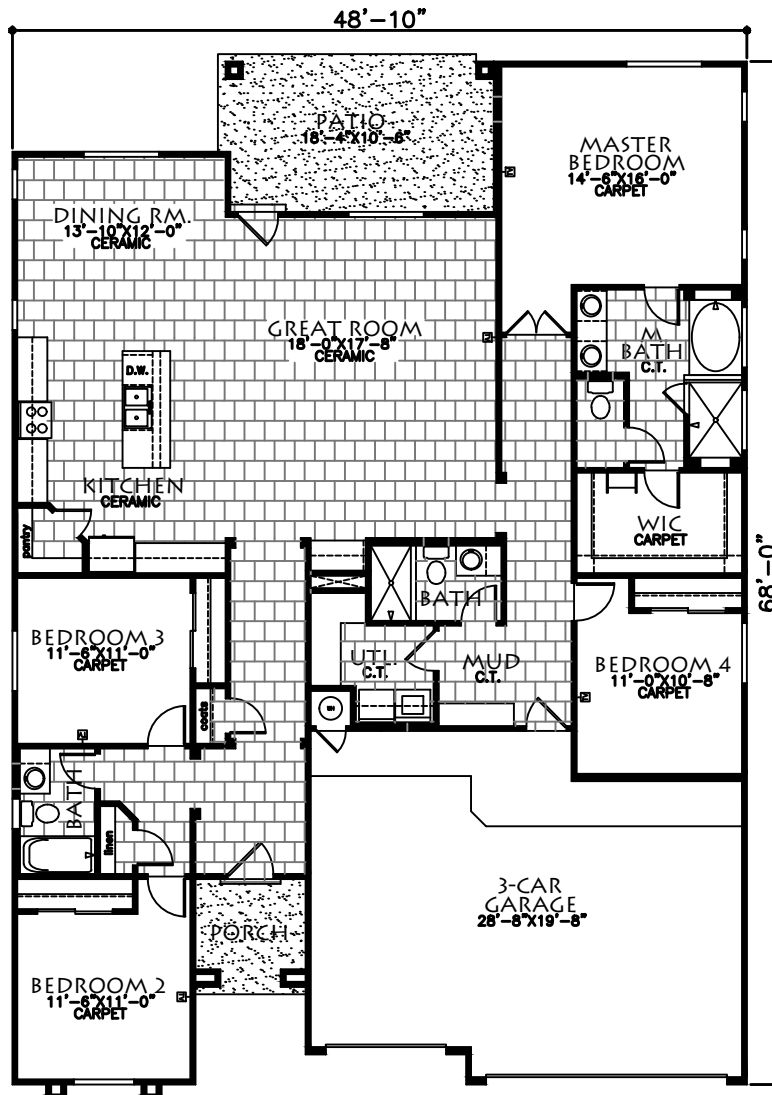
FLOOR PLAN
