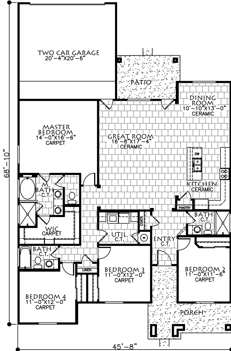
FLOOR PLAN
