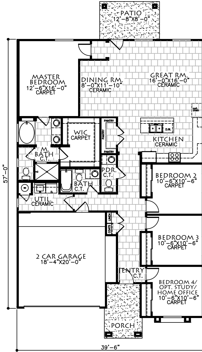
FLOOR PLAN
