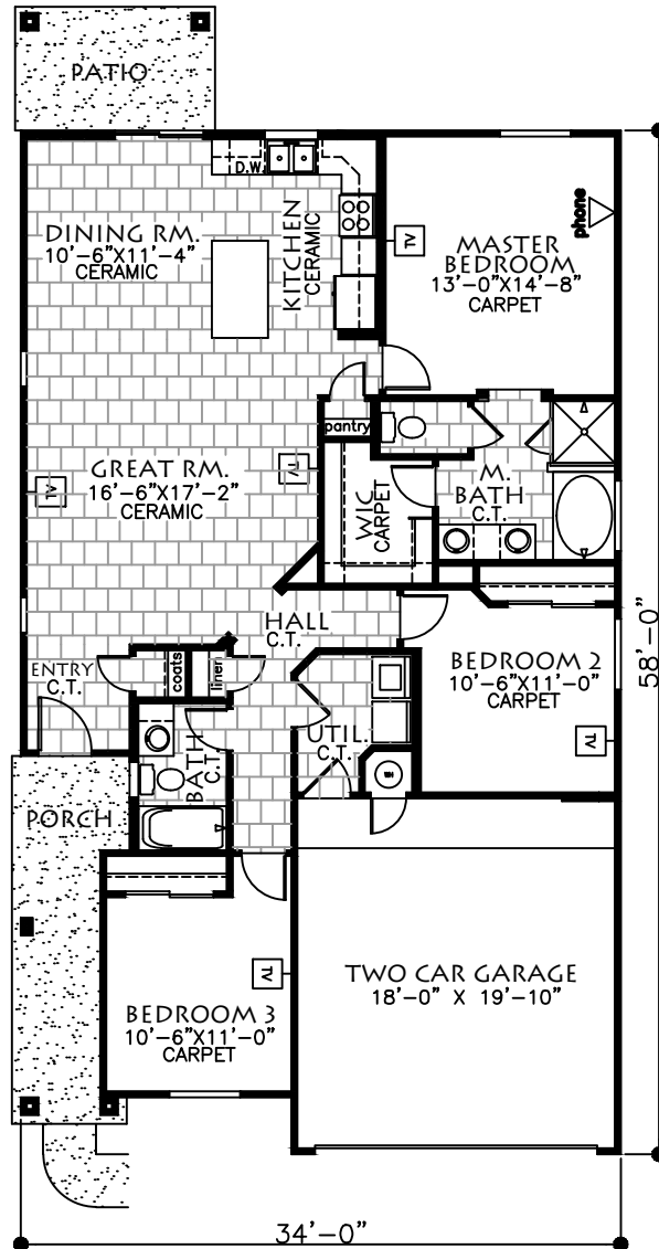
FLOOR PLAN
