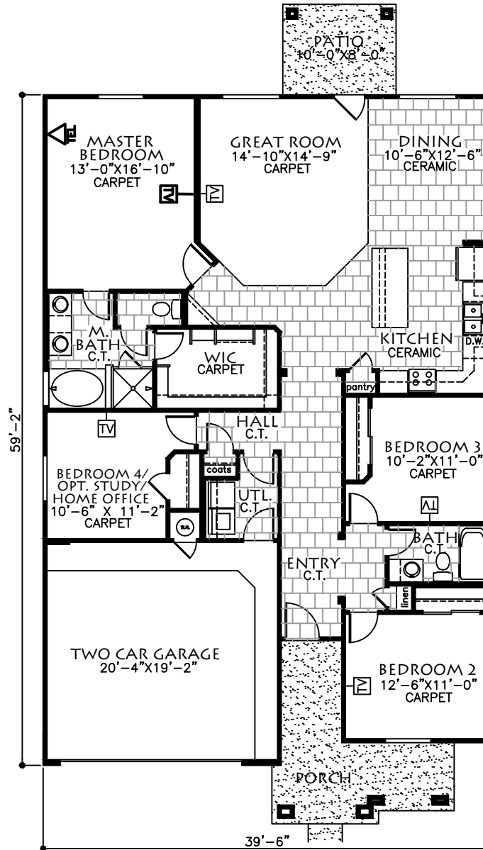
FLOOR PLAN
